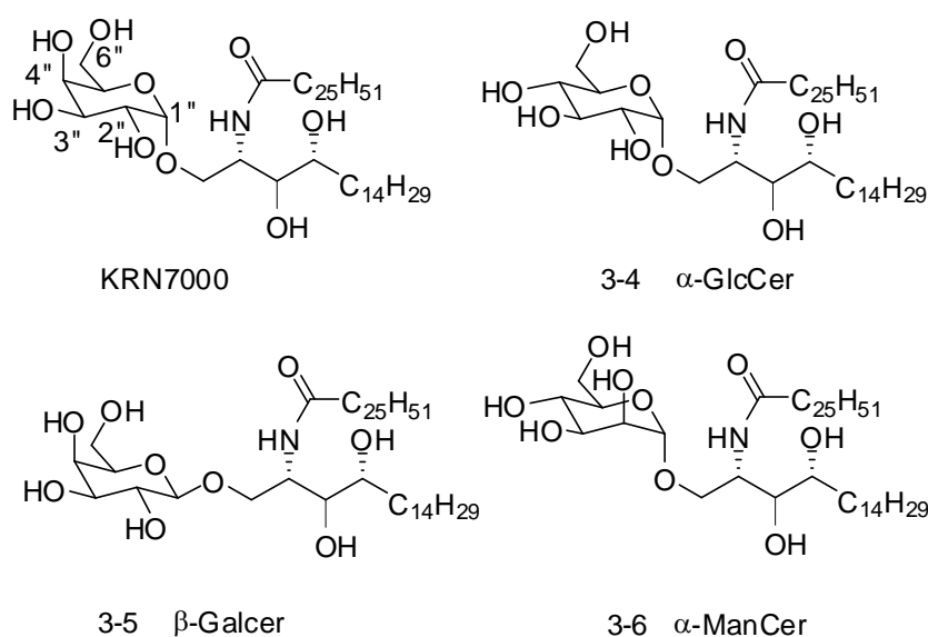
Figure 3.2. Structures of the compound 3-4 to 3-6.
